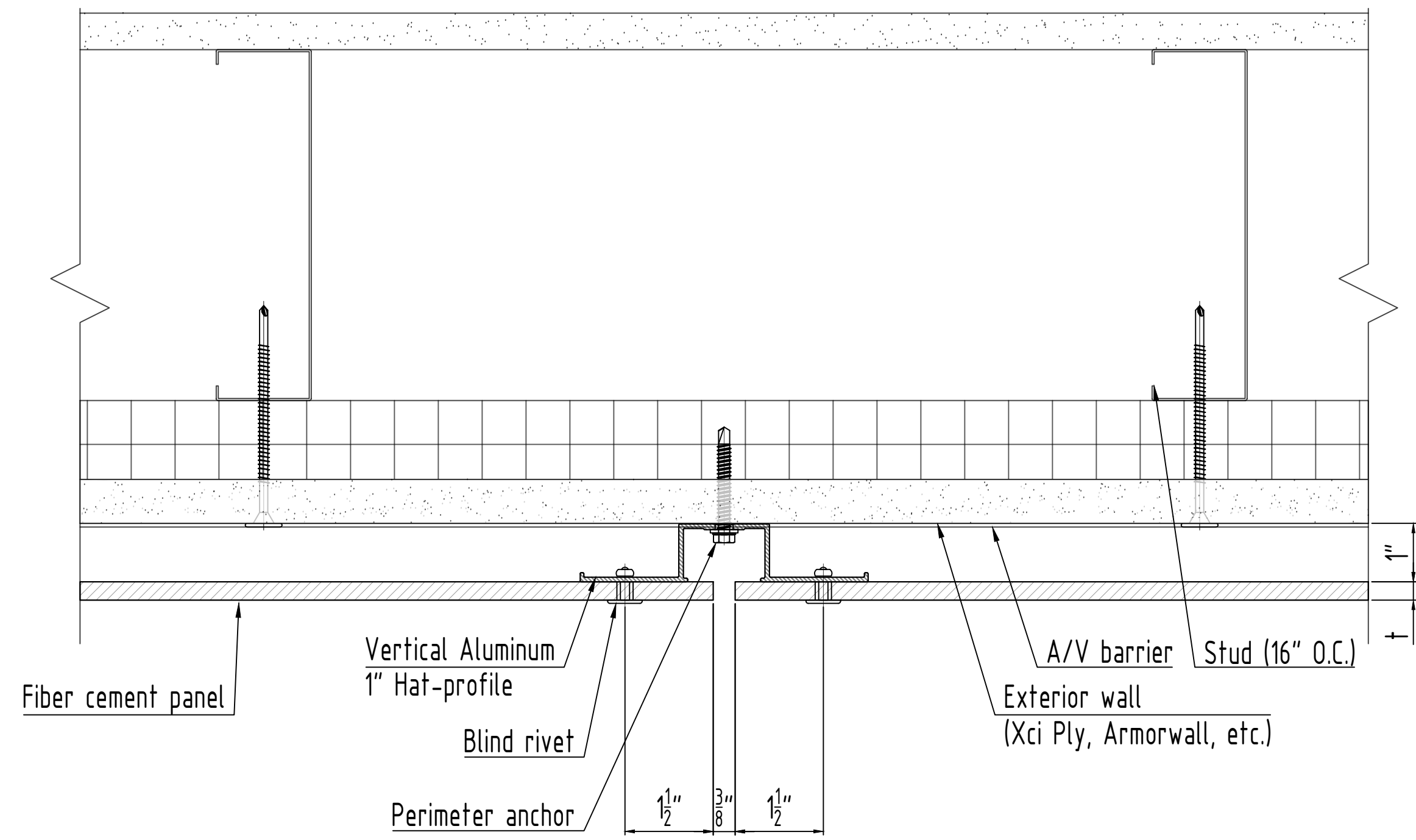
Typ. vertical joint (Option 1) 6" = 1'-0"
