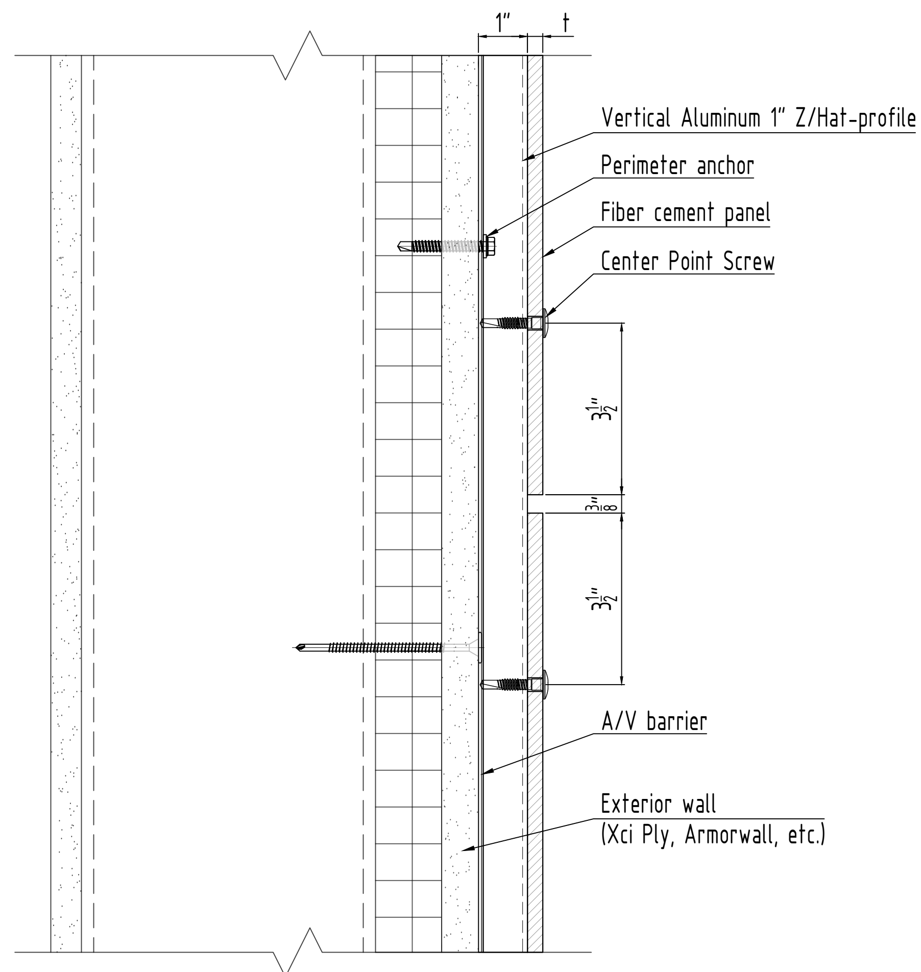
Typ. vertical joint (Option 1) 6" = 1'-0"
