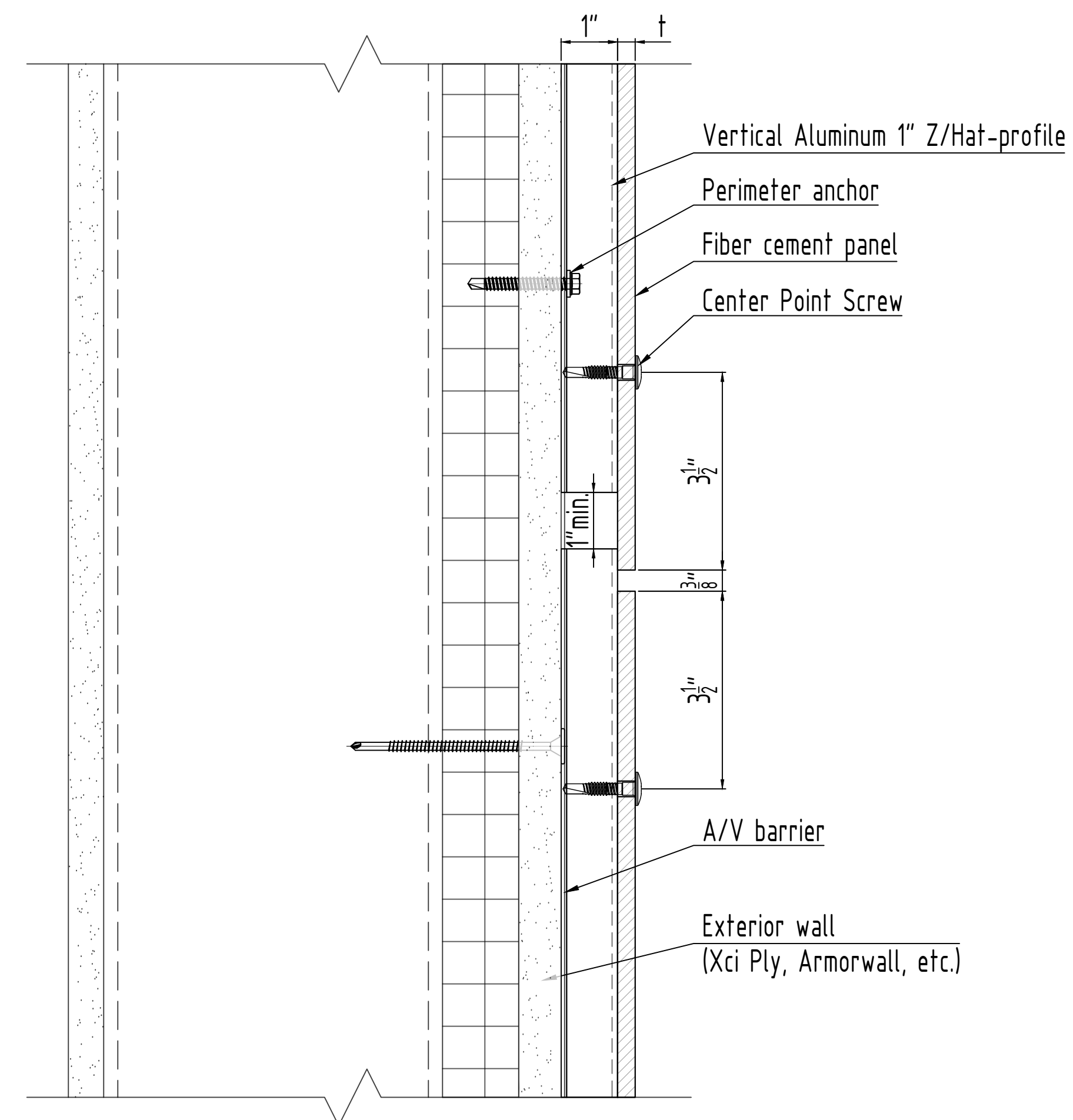
Typ. vertical joint (Option 2) 6" = 1'-0"
