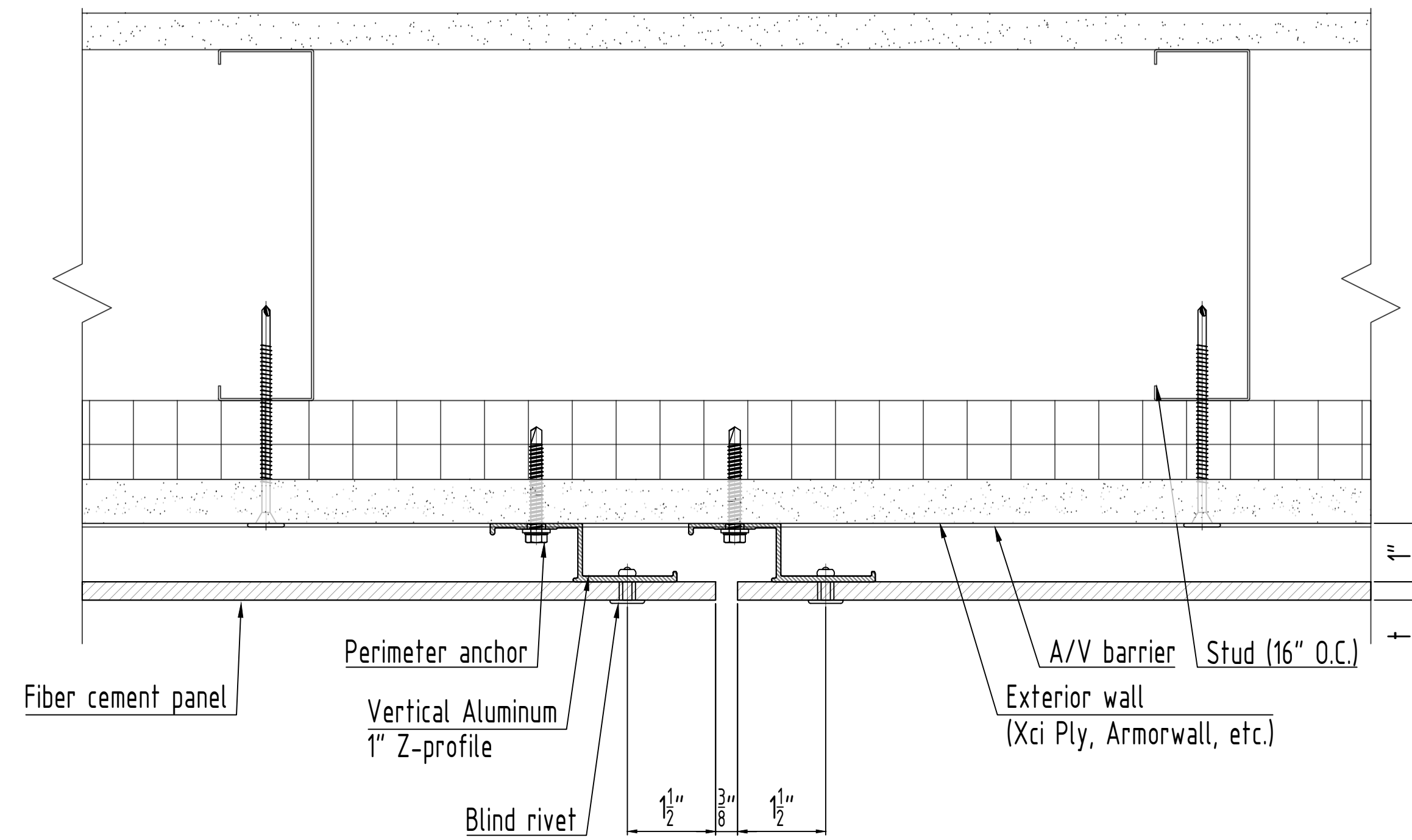
Typ. vertical joint (Option 2) 6" = 1'-0"
